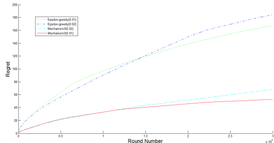
Figure 1: Accumulative regret
